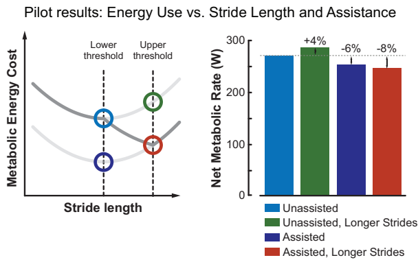
Fig. 4. Preliminary results from a test on a healthy subject, in which we sampled four points on the effort landscape: (Blue) Unassisted at Nominal stride length; (Green) Unassisted at Increased stride length; (Purple) Assisted at Nominal stride length; and (Red) Assisted at Increased stride length. During all conditions, subjects maintained a target stride length using visual feedback. During Assisted conditions, the robotic orthosis always provided maximal assistance. We found that voluntarily increasing stride length by 5% led to a 4% increase in energy cost. Applying robotic assistance reduced energy use by 6%. Doing both led to a net reduction of 8%.
